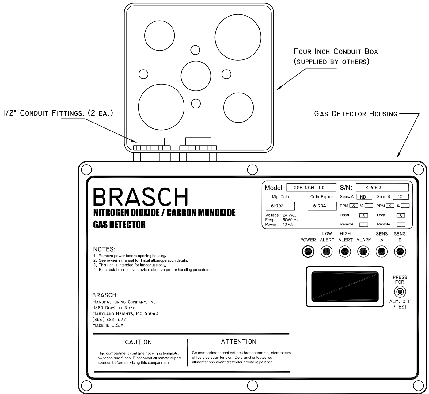
FIG. 6: MOUNTING VIEW GAS DETECTOR TO CONDUIT BOX
