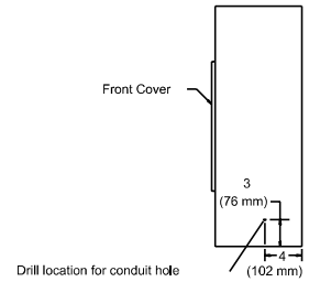
RIGHT SIDE VIEW (Typ. all lengths)
